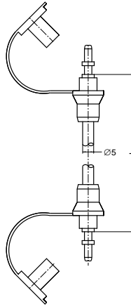
Test hose: SMA 1
