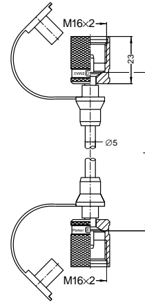
Test hose: SMA 3
