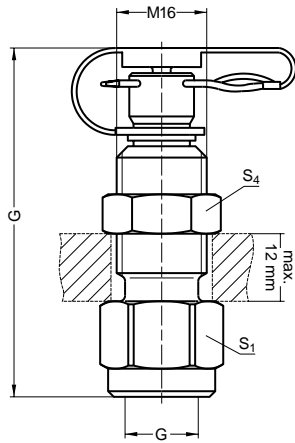
Pressure gauge connector: MAV-MA 1
