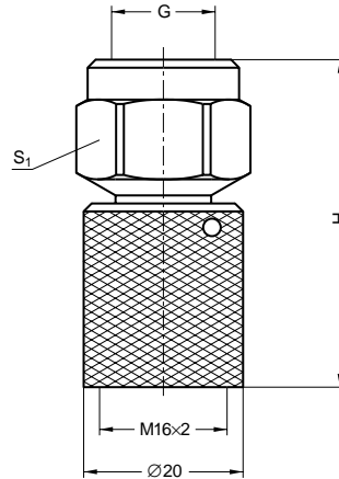
Manometer-Direct-Connector: MAVMD
