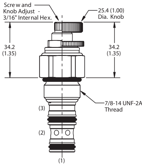
Screw/Knob Version
