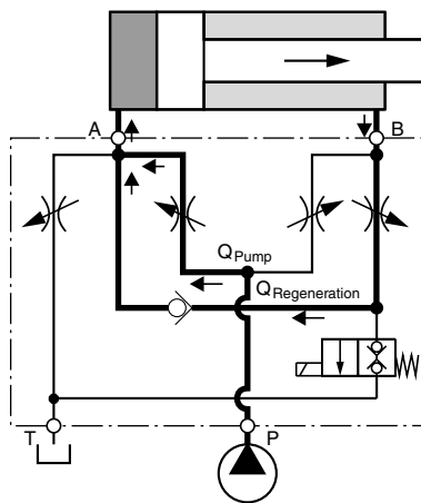
D*1FCZ (hybrid valve) Cylinder extending regenerative mode (high speed)
